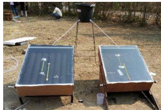
Fig 6: Experimental Set-Up
