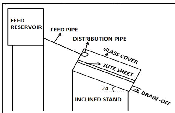
Fig 5: Set-Up for Solar Still
