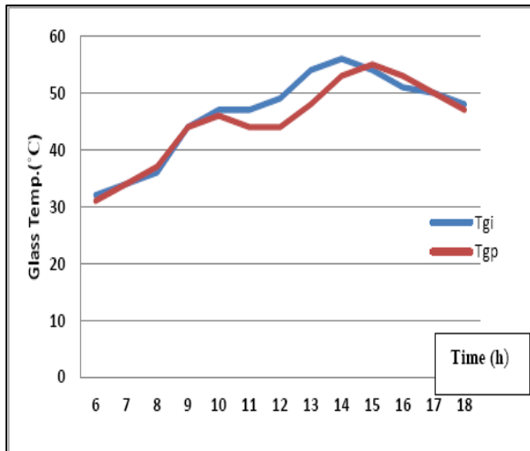
Fig 9: Variation of Glass Cover Temperature with Time
