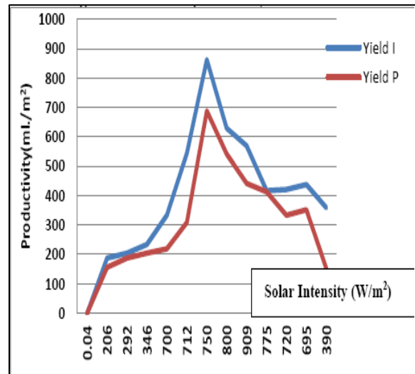
Fig 12: Variation of Productivity with Solar Intensity
