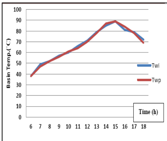
Fig 10: Variation of Basin Temperature with Time
